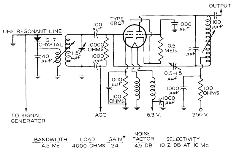
Fig. 13—Intermediate-preamplifier for ultra-high-frequency applications.
