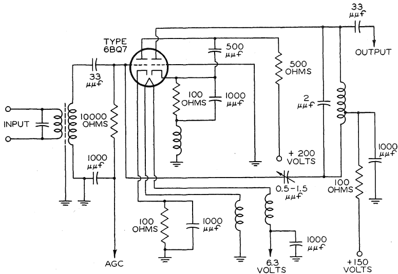
Fig. 11—Driven-grounded-grid circuit.
